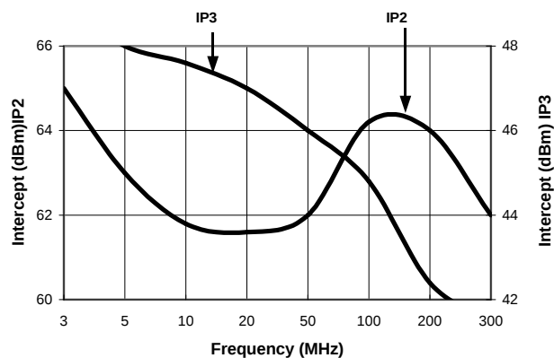
Intermodulation Intercept
