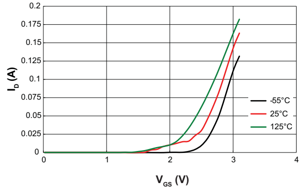
Transfer Characteristics
