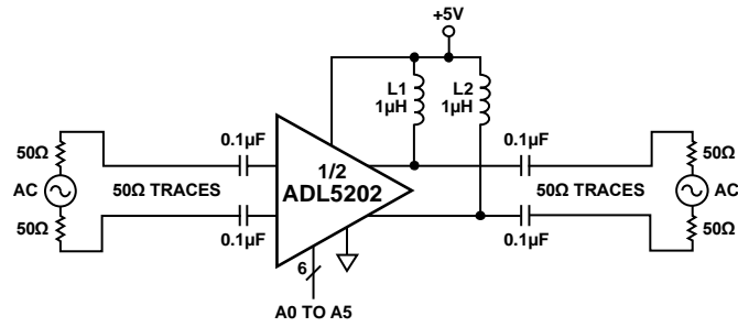
Figure 47. Test Circuit for S-Parameters on Dedicated 50 \Omega Differential-to-Differential Board
