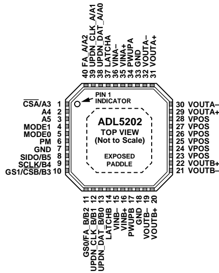
Figure 5. Pin Configuration
