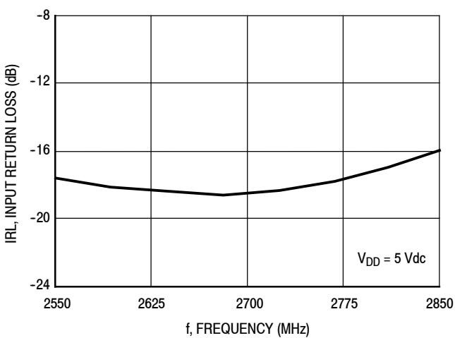
Figure 22. Input Return Loss (S11) versus Frequency
