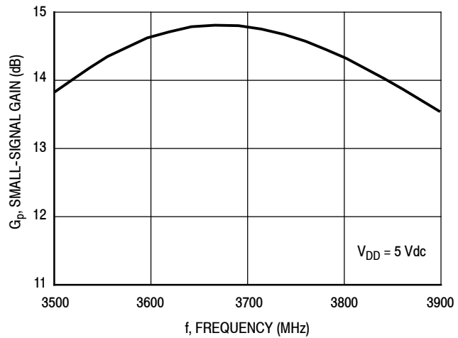
Figure 45. Small-Signal Gain (S21) versus Frequency
