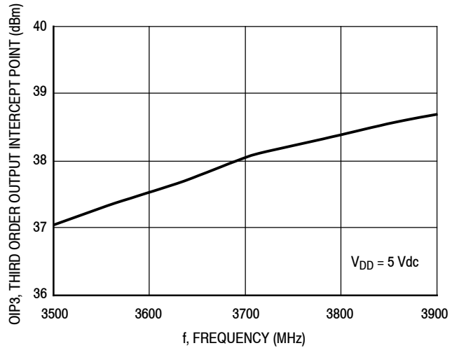
Figure 49. Third Order Output Intercept Point versus Frequency
