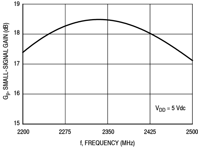
Figure 29. Small-Signal Gain (S21) versus Frequency
