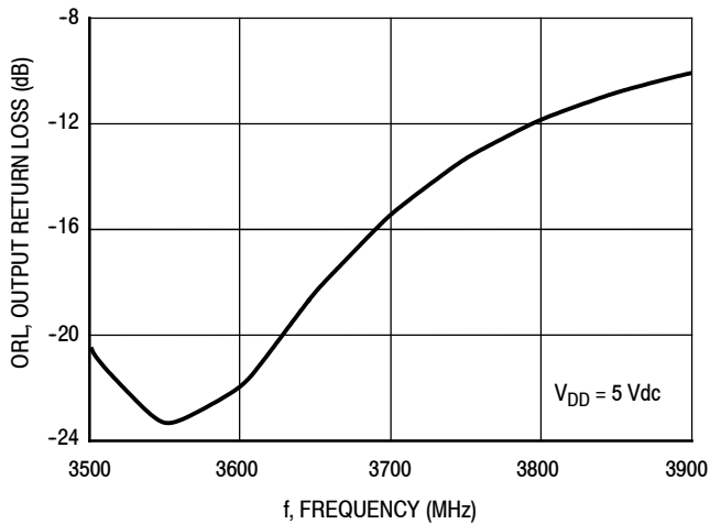
Figure 47. Output Return Loss (S22) versus Frequency
