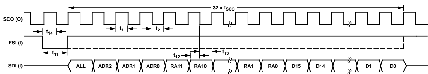
Figure 3. Register Write
