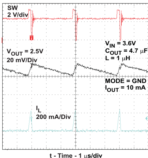
Figure 33. PFM Mode Operation I_{OUT} = 10mA
