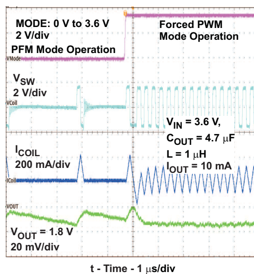
Figure 38. Mode Transition PFM / Forced PWM Mode
