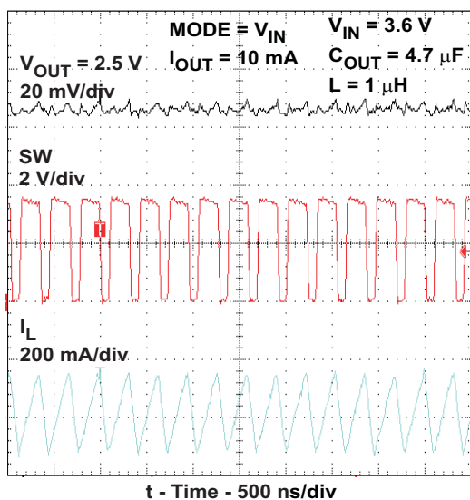
Figure 35. Forced PWM Mode Operation I_{OUT} = 10mA
