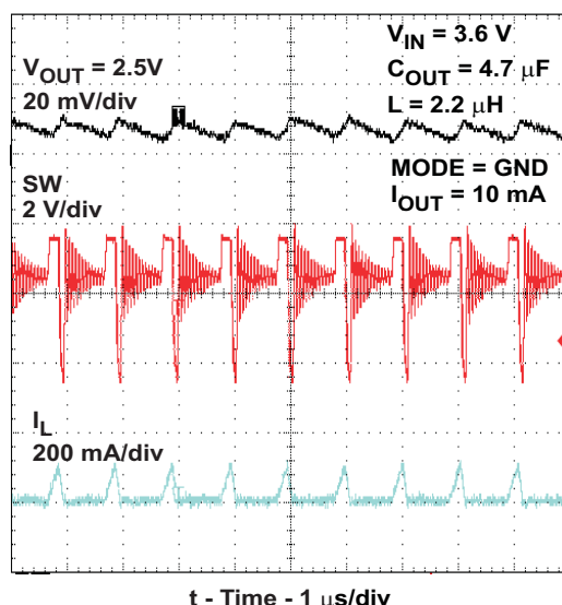
Figure 34. PFM Mode Operation I_{OUT} = 10mA
