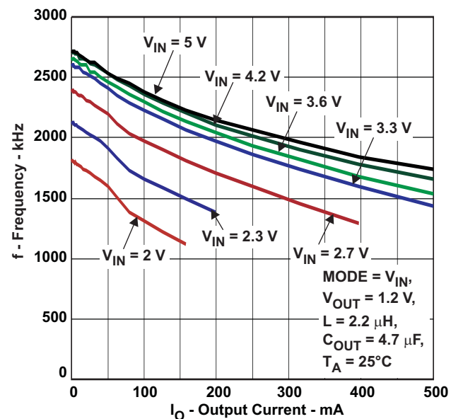
Figure 24. Switching Frequency vs Output Current, 1.2V Output Voltage MODE = V_{IN}
