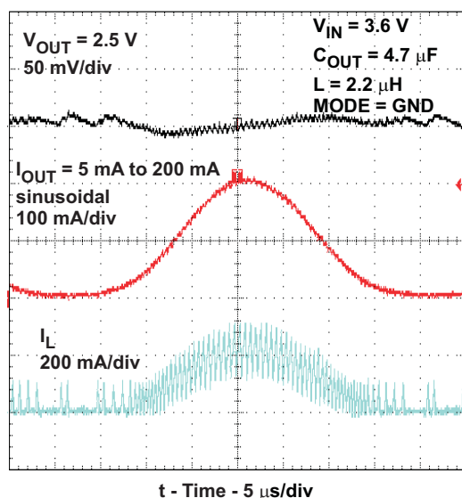
Figure 39. AC – Load Regulation Performance 2.5V VOUT PFM Mode
