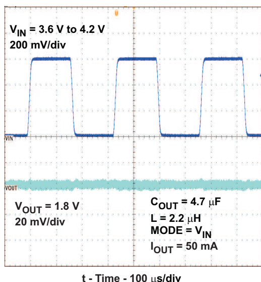
Figure 37. Line Transient Response PWM Mode
