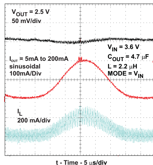
Figure 40. AC – Load Regulation Performance 2.5V VOUT PWM Mode
