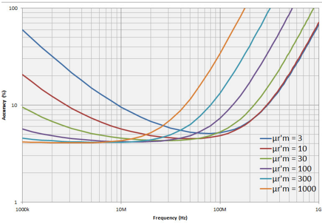
Figure 46. Permeability accuracy ( \frac{\Delta\mu'}{\mu'} ) vs. frequency (at F = 3 mm, typical)
