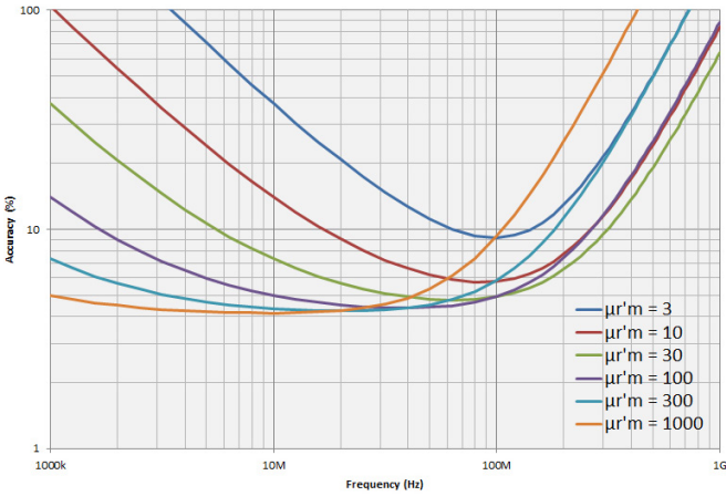
Figure 45. Permeability accuracy ( \frac{\Delta\mu'}{\mu'} ) vs. frequency (at F = 0.5 mm, typical)
