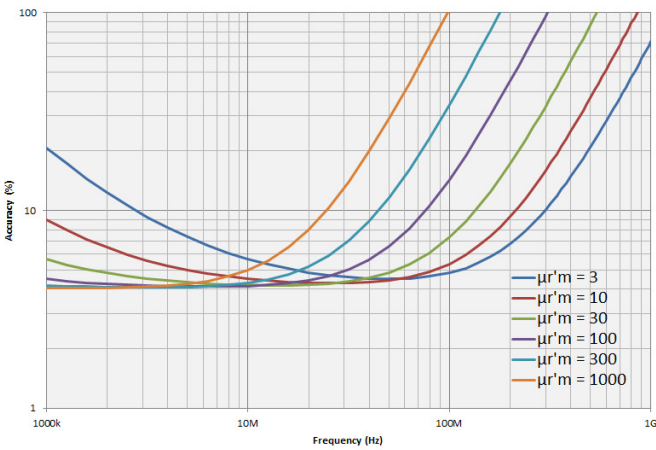
Figure 47. Permeability accuracy ( \frac{\Delta\mu'}{\mu'} ) vs. frequency (at F = 10 mm, typical)
