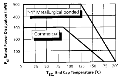
FIGURE 3 Power Derating Curve
