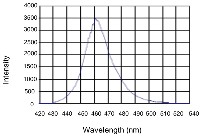
Fig.5 Relative Intensity vs. Wavelength (Ta=25°C)
