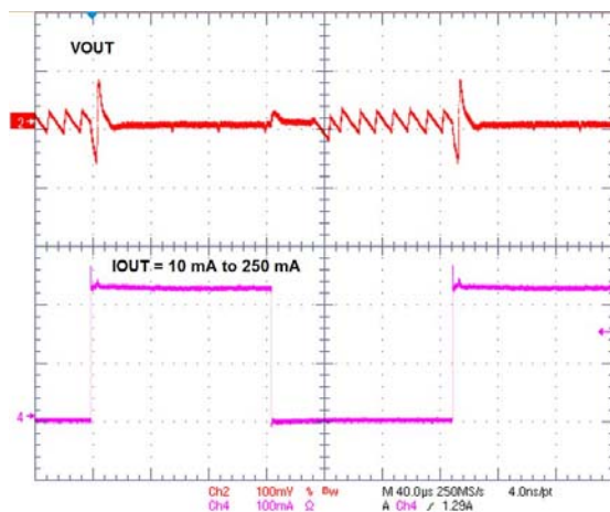
Figure 44. Load Transient Response I_{OUT} = 10\text{ to } 250\text{ mA} , V_{OUT} = 2.5\text{ V}
