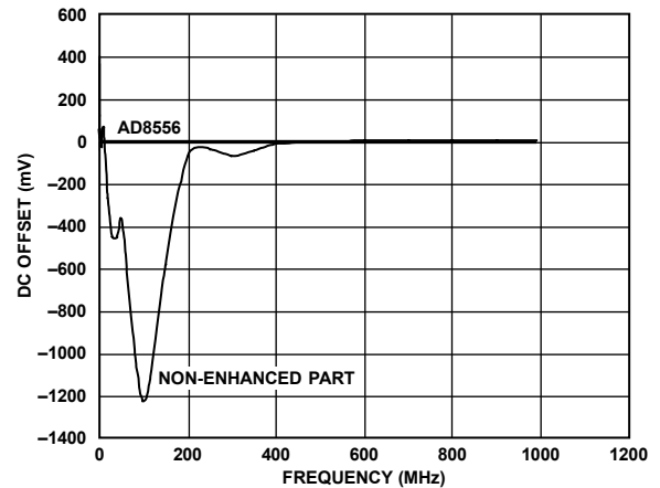
Figure 55. Response of AD8556 to EMI/RFI Differential Signals
