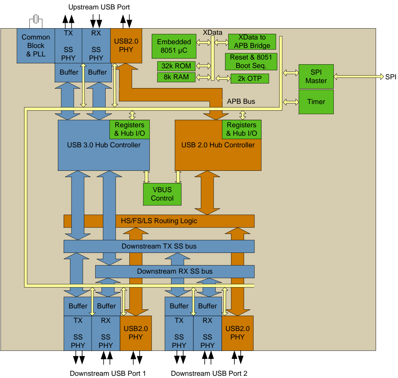
FIGURE 2-1: USB5532B BLOCK DIAGRAM
