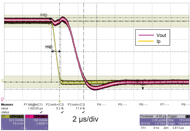
Figure 8: Step response
