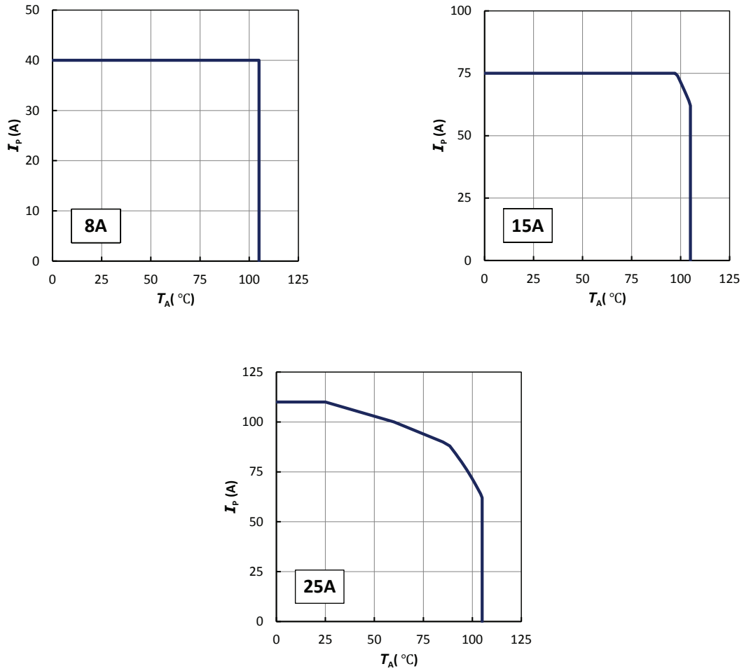
Figure 16: I_p vs T_A for HO series
