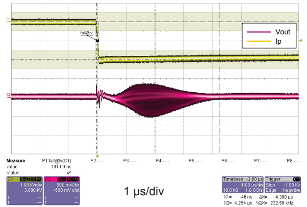
Figure 4: dv/dt
