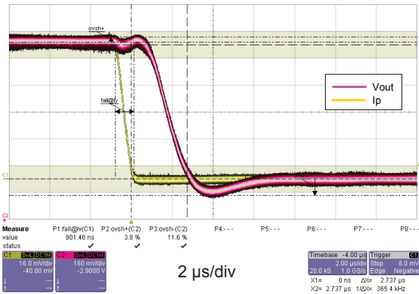
Figure 3: Step response
