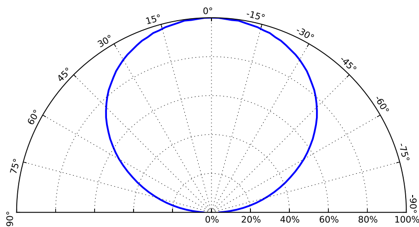
Figure 6. Typical polar radiation pattern for LUXEON TX at 700mA, Tj=85°C.
