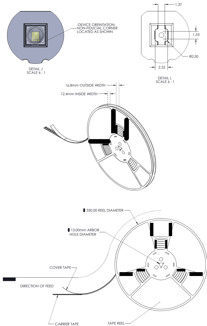
Figure 13. Reel dimensions for LUXEON TX.
