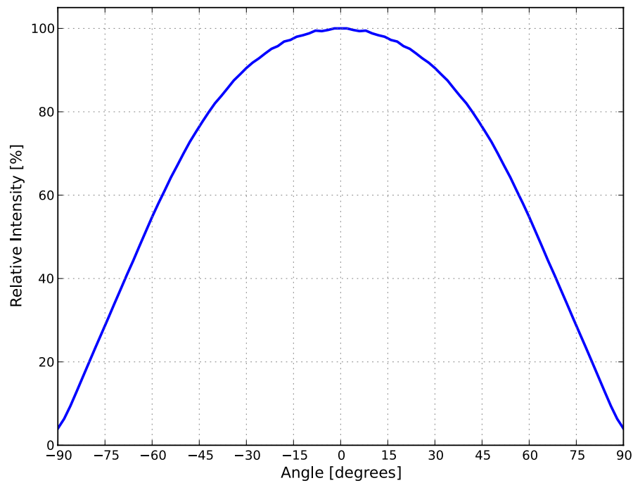
Figure 5. Typical radiation pattern for LUXEON TX at 700mA, Tj=85°C.
