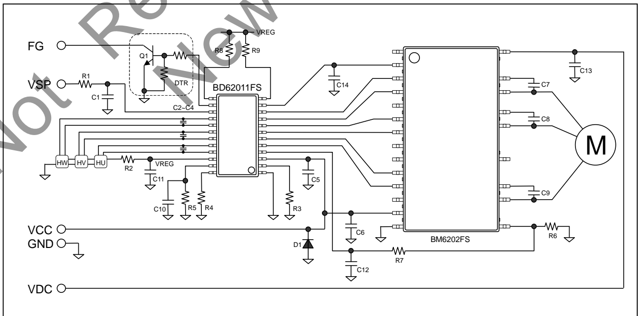
Figure 1. Application circuit example - BD62011FS & BM6202FS
