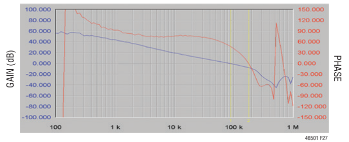
Figure 27. Bode Plot of Figure 23 Circuit
