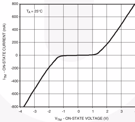
Fig. 7 On-State Characteristics
