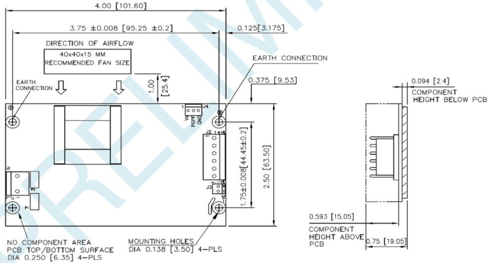
Mechanical Drawing – Option 1 with PGPF
