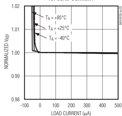
REFERENCE VOLTAGE CHANGE vs. LOAD CURRENT
