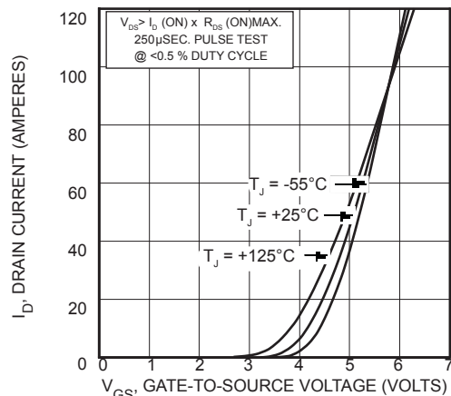
FIGURE 3, TRANSFER CHARACTERISTICS
