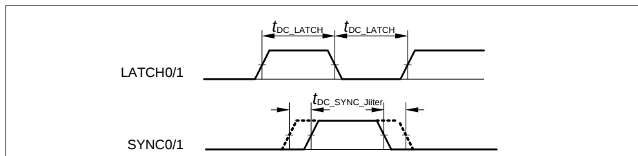
Figure 59 Sync/Latch Timings
