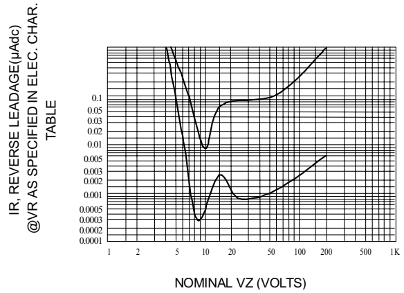
Fig. 3-TYPICAL REVERSE LEAKAGE
