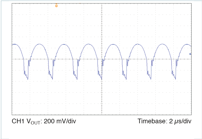
Figure 19 — Output voltage ripple, V_{IN} = 270\text{ V} , V_{OUT} = 5.0\text{ V} , C_{OUT\_EXT} = 1000\text{ }\mu\text{F} , R_{LOAD} = 0.100\text{ }\Omega
