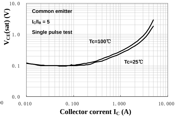
Saturation Voltage
