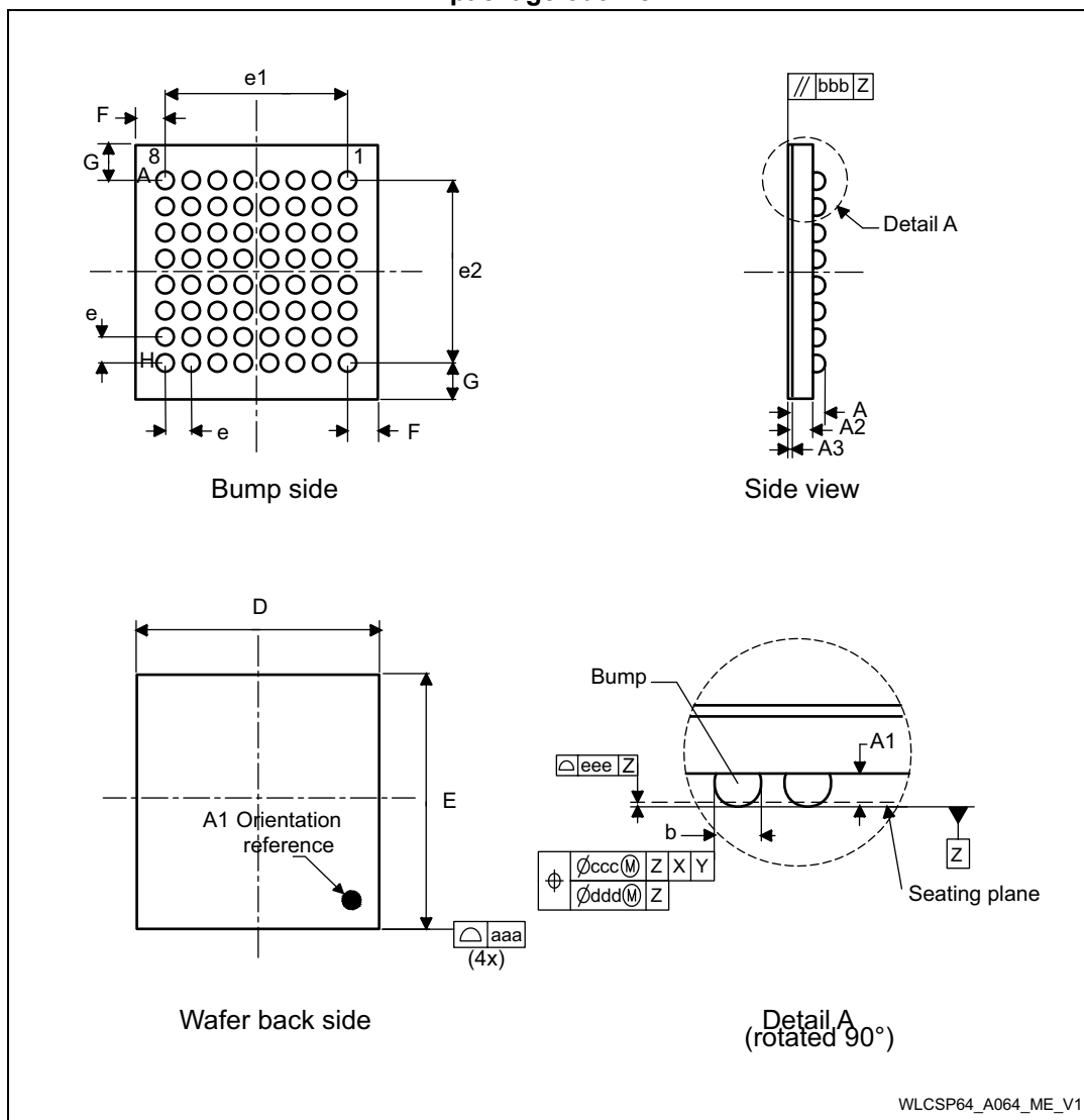
Figure 53. WLCSP64 - 64-ball, 3.141 x 3.127 mm, 0.35 mm pitch wafer level chip scale package outline
