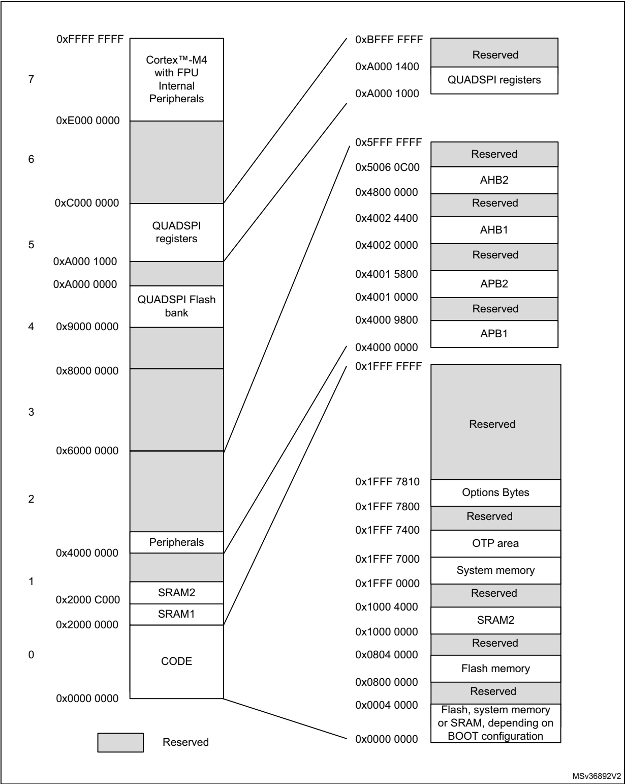
Figure 13. STM32L443xx memory map
