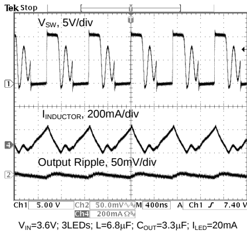
Fig. 10 Operation Waveform
