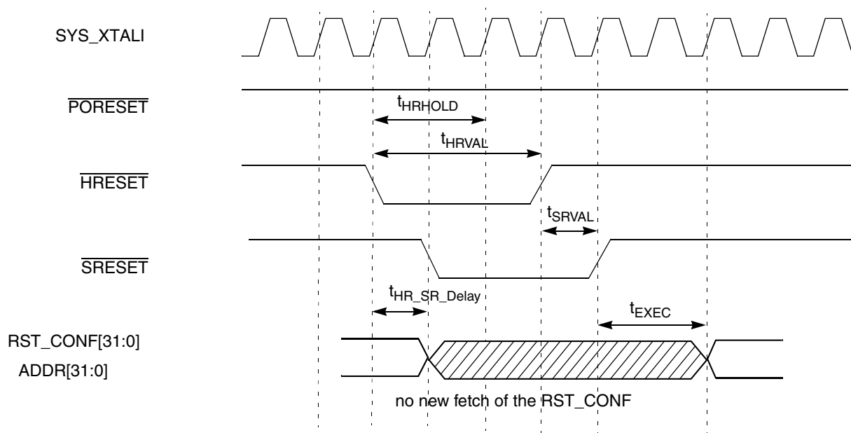
Figure 5. HRESET Behavior
