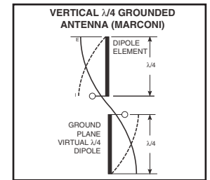
Figure 29: Dipole Antenna
