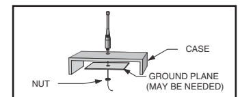
Figure 30: Remote Ground Plane
