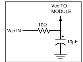
Figure 19: Supply Filter
