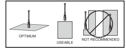
Figure 28: Ground Plane Orientation
