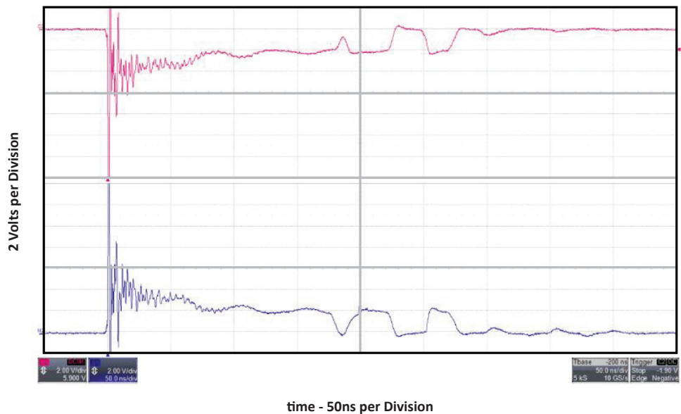
FIGURE 3 8kV POSITIVE & NEGATIVE ESD CLAMPING WAVEFORM
