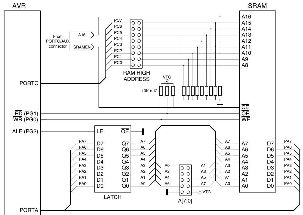
Figure 2-10. SRAM Block Schematic
