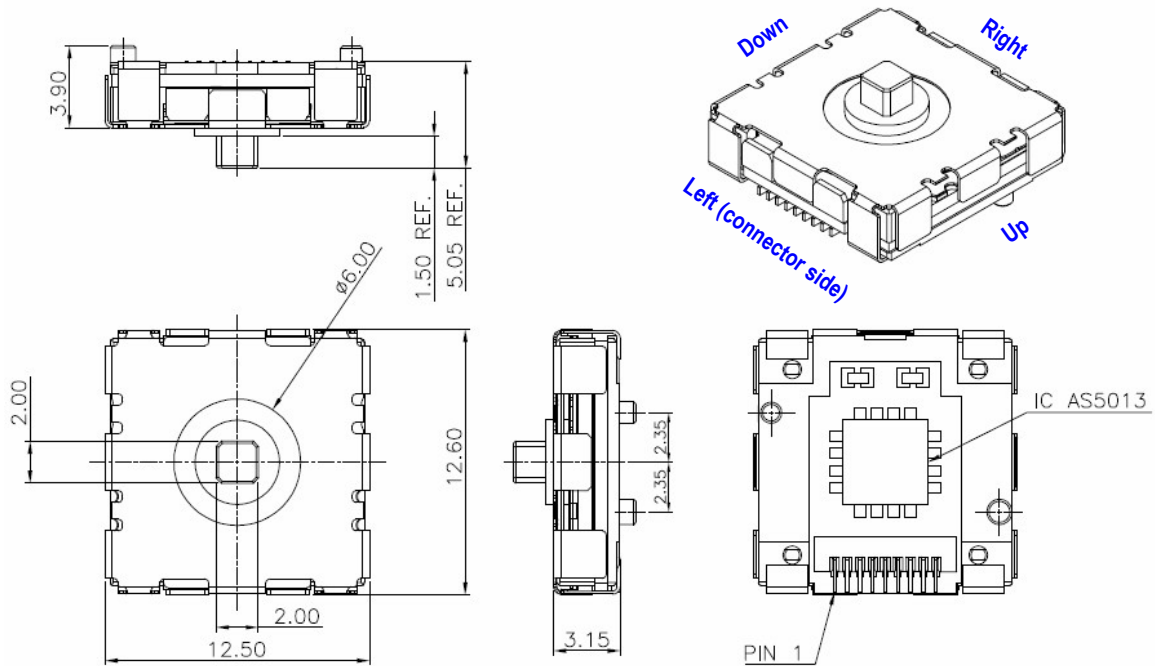
Figure 18. N40P112 Dimensions (mm \pm 0.15 )
