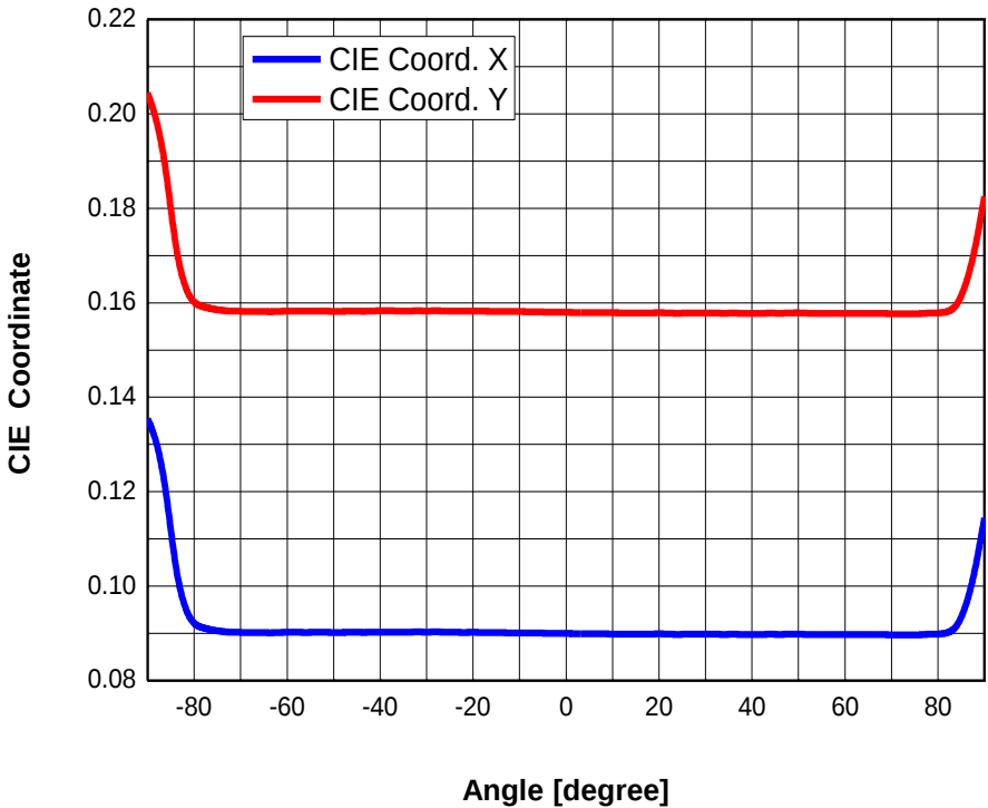
Fig 10. Color. vs. Viewing Angle, T_j = 25^{\circ} C, I_F=10 mA
