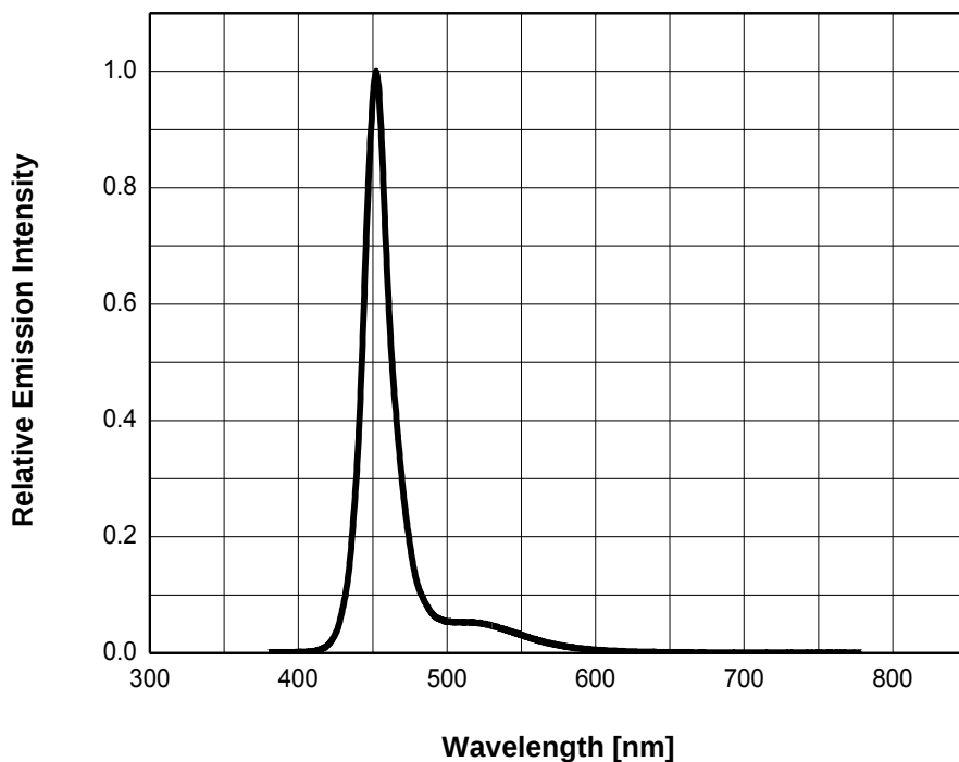
Fig 1. Color Spectrum, I_F = 10\text{mA} , T_j = 25^\circ\text{C} , RH30%
