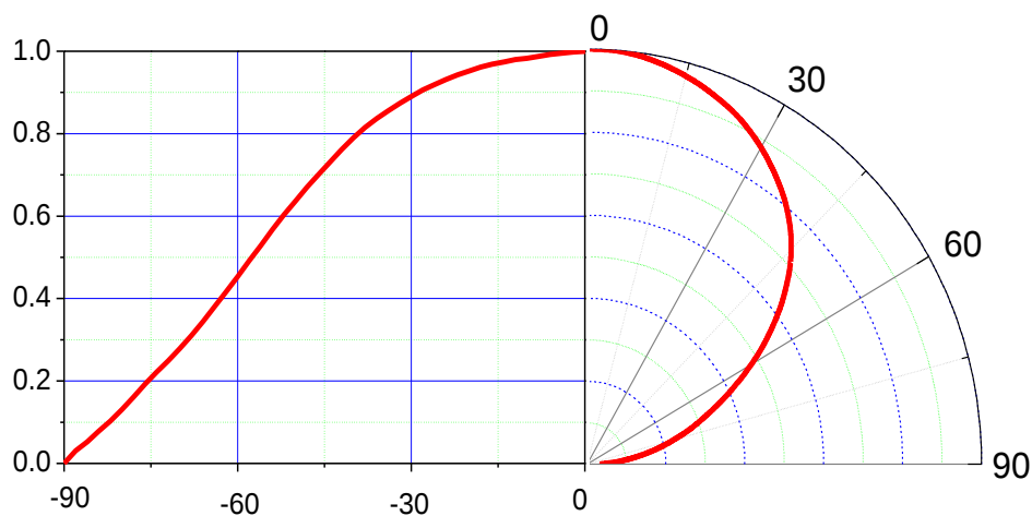
Fig 2. Viewing Angle Distribution, I_F = 10\text{mA}
