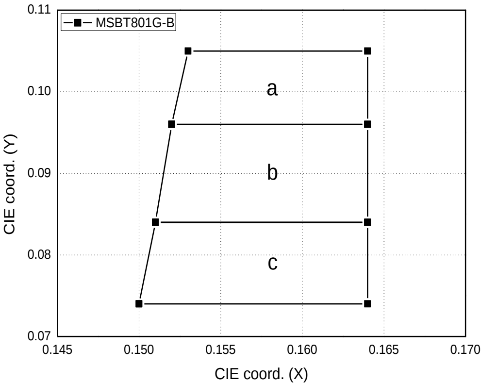
CIE Chromaticity Diagram, I_F = 10\text{mA} , T_j = 25^\circ\text{C}
