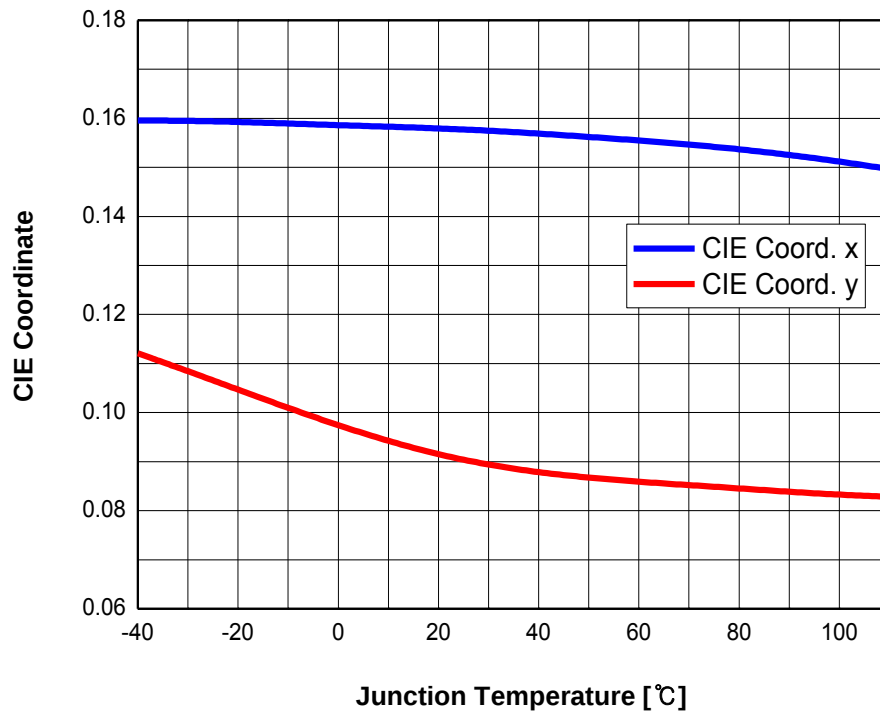
Fig 8. Chromaticity Coordinate vs. Junction Temperature, I_F = 10\text{mA}
