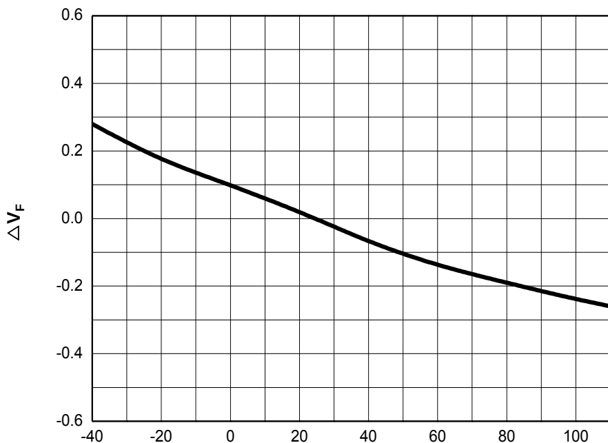
Fig 7. Junction Temperature vs. Forward Voltage shift, I_F = 10\text{mA}
