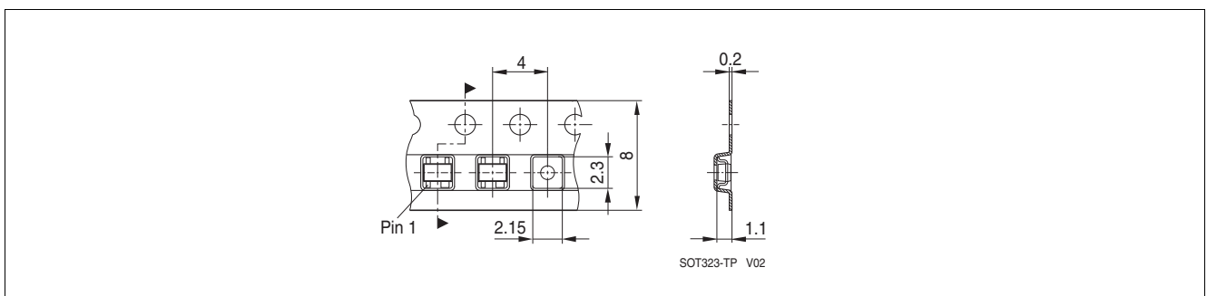
Figure 7-4 Tape Dimensions
