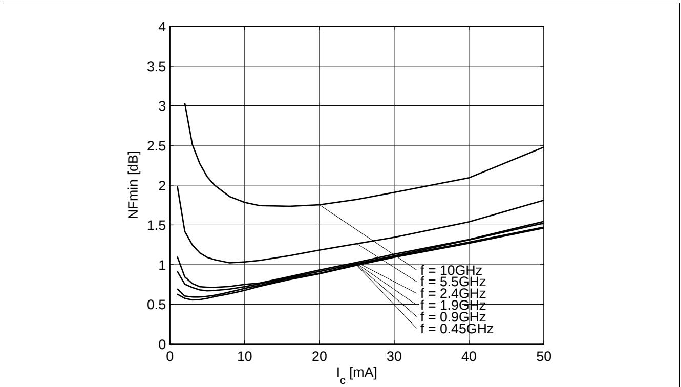
Figure 5-17 Noise Figure NF_{min} = f(I_c) , V_{CE} = 3\text{ V} , Z_S = Z_{opt} , f = Parameter in GHz
