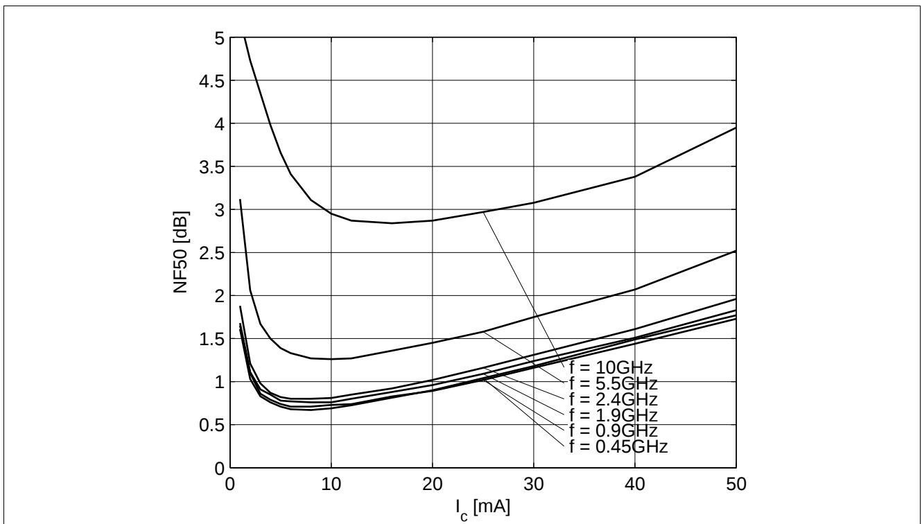
Figure 5-18 Noise Figure NF_{50} = f(I_c) , V_{CE} = 3\text{ V} , Z_S = 50\ \Omega , f = Parameter in GHz
