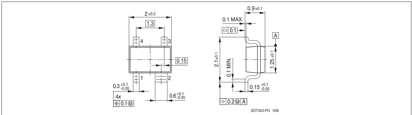
Figure 7-1 Package Outline
