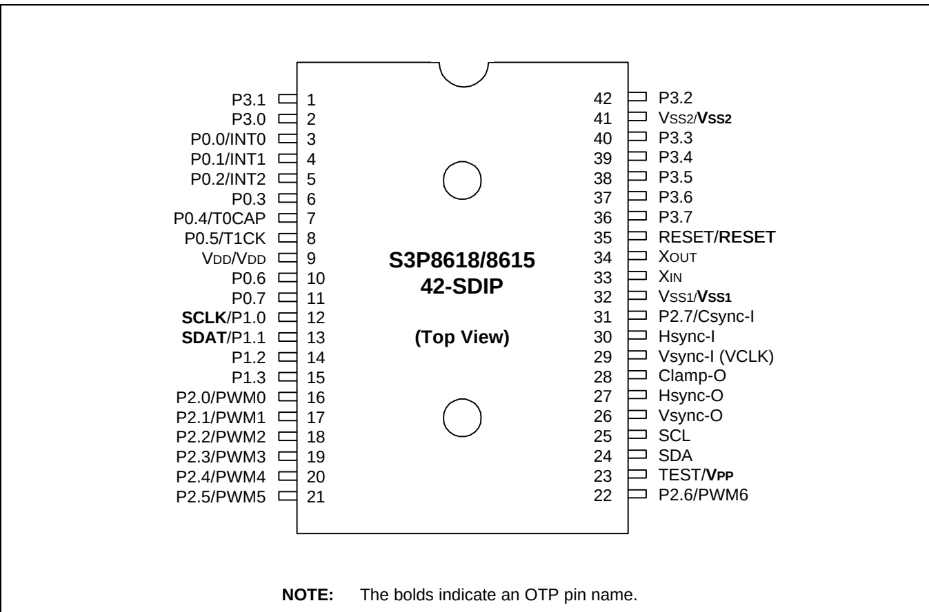
Figure 18-1. S3P8615 Pin Assignments (42-SDIP Package)
