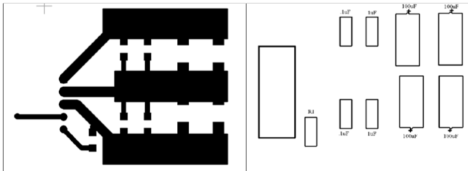
Fig. 2a. Layer 1 conductor. Ground plane below layer 1
