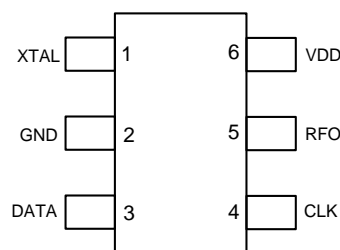
CMT2110/17AW
