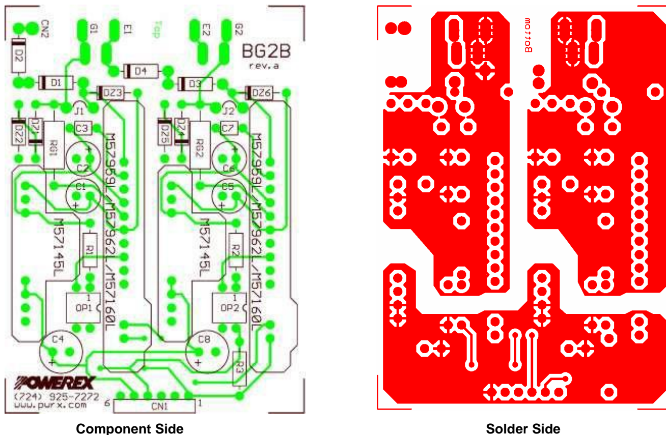
Figure 5: BG2B Printed Circuit Board Layout
