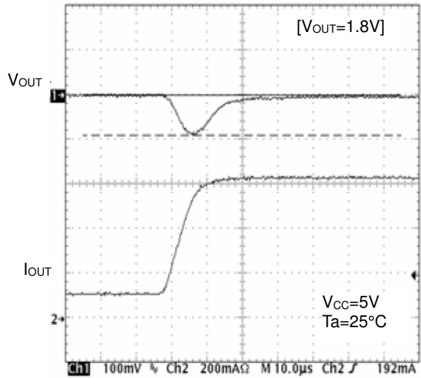
Figure 23. Transient Response ( I_o=100mA to 600mA , 10\mu s )
