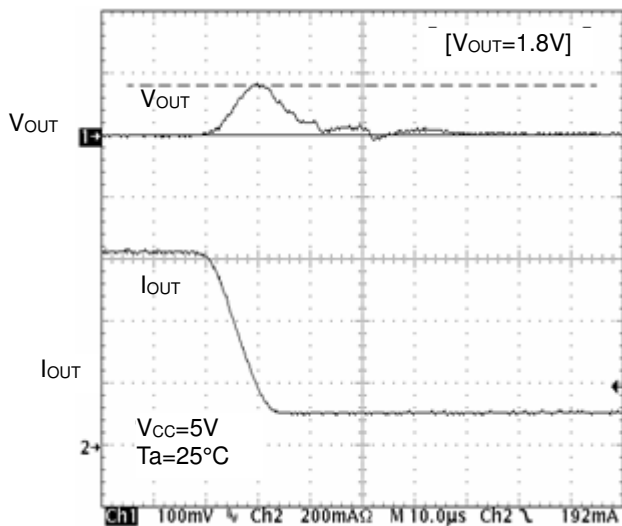
Figure 24. Transient response ( I_o=600mA to 100mA , 10\mu s )
