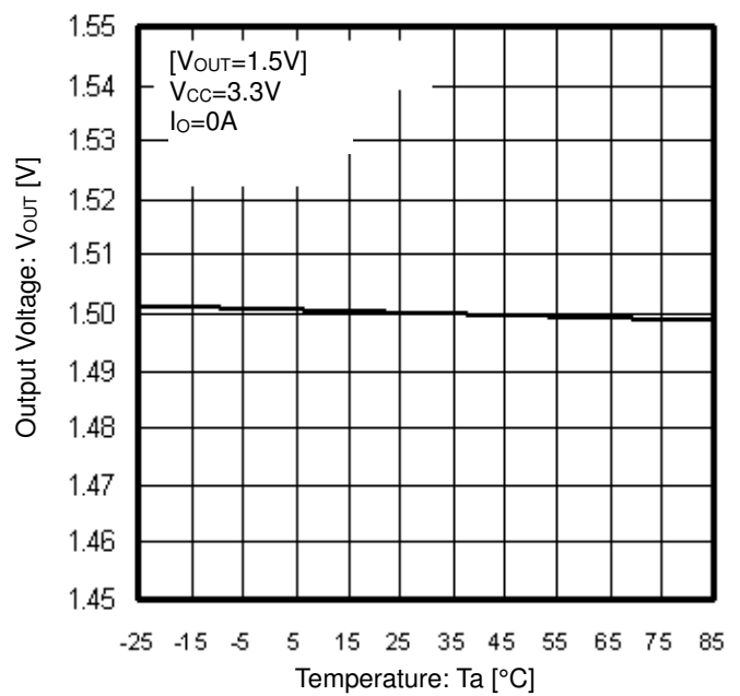
Figure 73. Output Voltage vs Temperature
