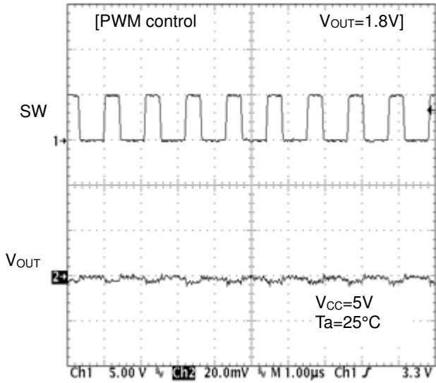
Figure 22. SW Waveform ( I_o=200mA )
