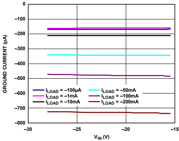
Figure 45. Ground Current vs. Input Voltage ( V_{IN} ), Adjustable Output Voltage, V_{OUT} = -15 V
