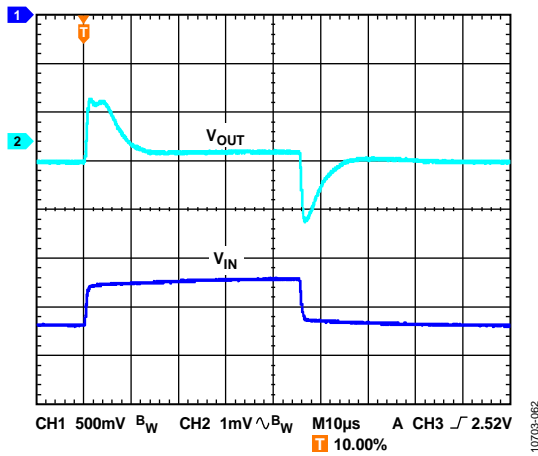
Figure 64. Line Transient Response, 500 mV Step, V_{OUT} = -1.22\text{ V} , I_{LOAD} = -200\text{ mA}
