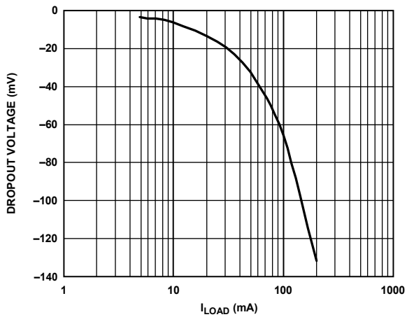
Figure 46. Dropout Voltage vs. Load Current ( I_{LOAD} ), Adjustable Output Voltage, V_{OUT} = -15 V
