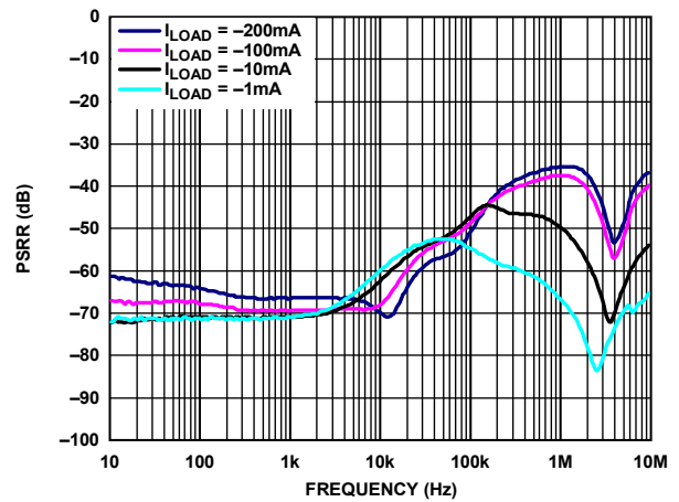
Figure 49. Power Supply Rejection Ratio (PSRR) vs. Frequency, V_{OUT} = -1.22 V vs. Different Load Currents ( I_{LOAD} ), V_{IN} = -2.7 V
