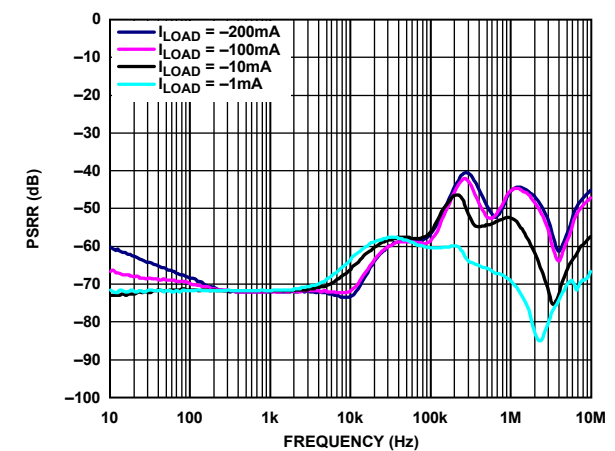
Figure 50. Power Supply Rejection Ratio (PSRR) vs. Frequency, V_{OUT} = -1.22 V vs. Different Load Currents ( I_{LOAD} ), V_{IN} = -5.7 V
