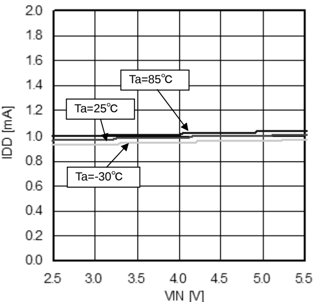
Figure 5. Circuit current
