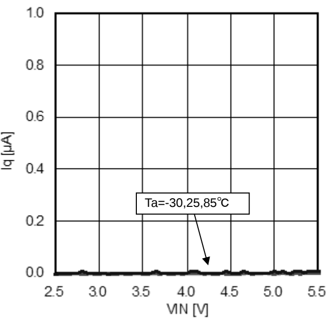
Figure 4. Quiescent Current
