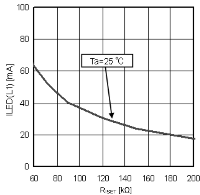
Figure 12. LED current vs. R_{ISET} (VIN = 3.6 V, at the maximum current setting)
