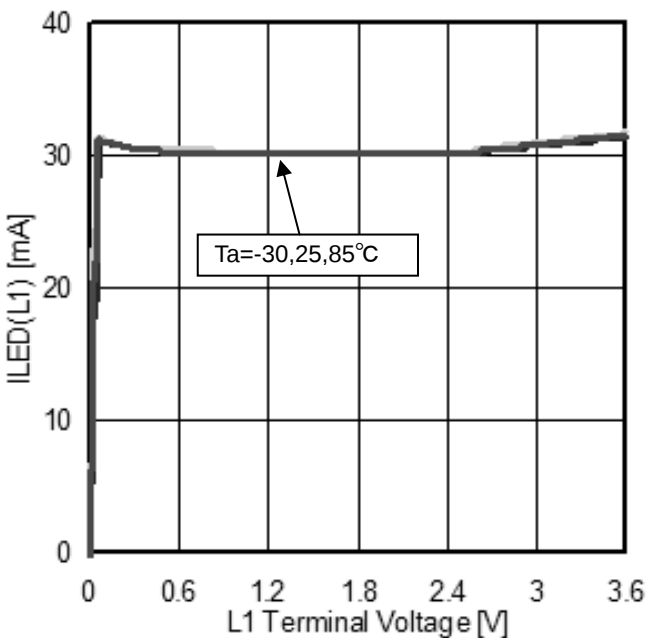
Figure 7. LED output current vs. LED pin voltage ( V_{IN} = 3.6 V , at 32 mA of LED current)
