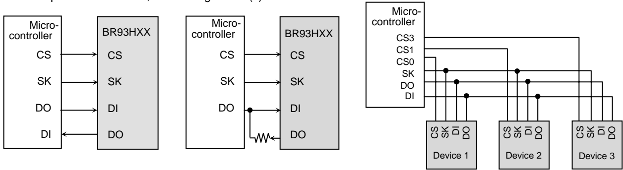
Figure 27-(a) Connection by 4 lines
