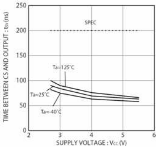
Figure 23. Time from CS to output establishment t SV
