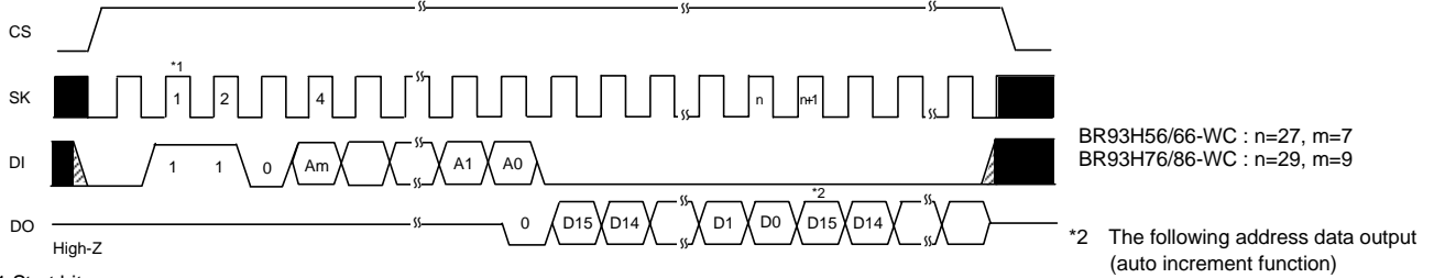
Figure 28. Read cycle
