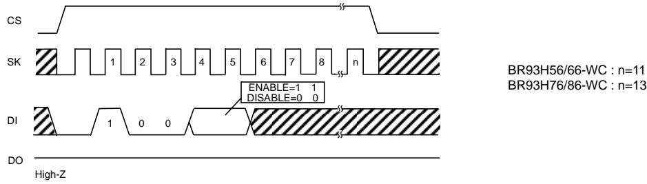
Figure 31. Write enable (WEN) / disable (WDS) cycle
