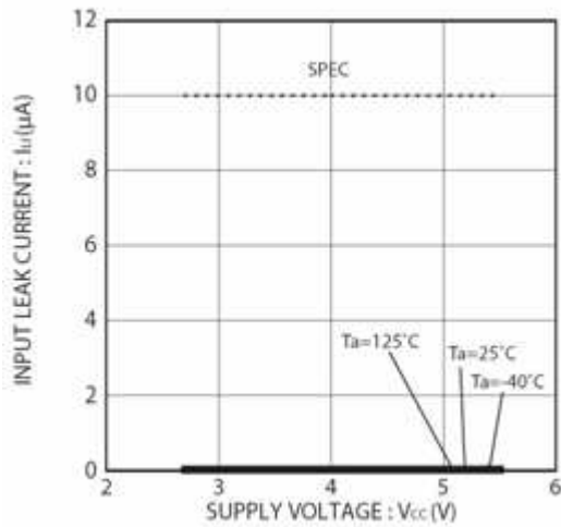
Figure 7. Input leak current I_{ILI} (CS, SK, DI)
