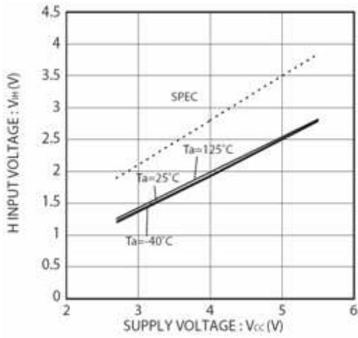
Figure 1. H input voltage VIH (CS, SK, DI)
