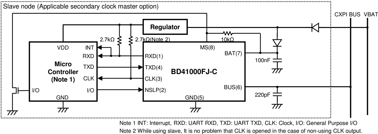
Figure 19. Application Example of Secondary Clock Master Option
