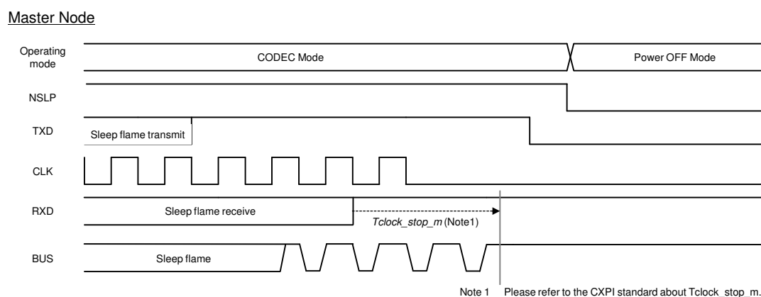
Figure 6. The Timing Chart from “Normal Mode” to “Sleep Mode” (Master)
