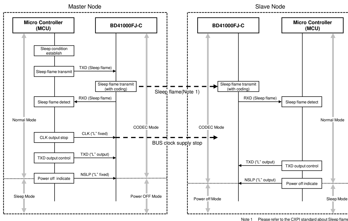
Figure 5. The Sequence from “Normal Mode” to “Sleep Mode”
