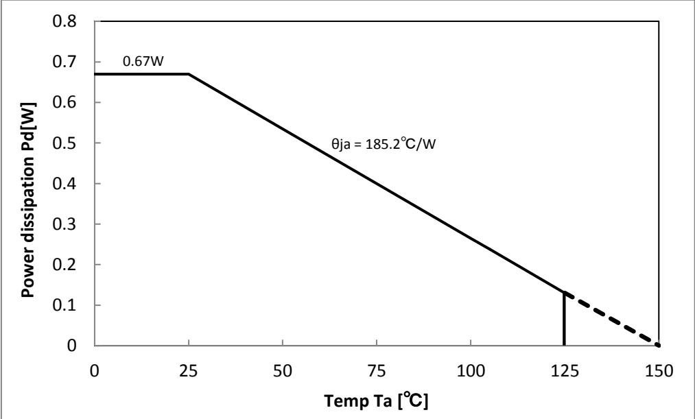
Figure 20. Power Dissipation
