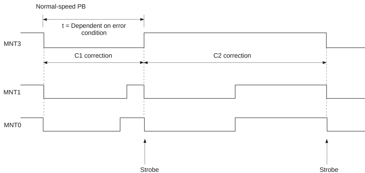
Timing Chart 3-3
