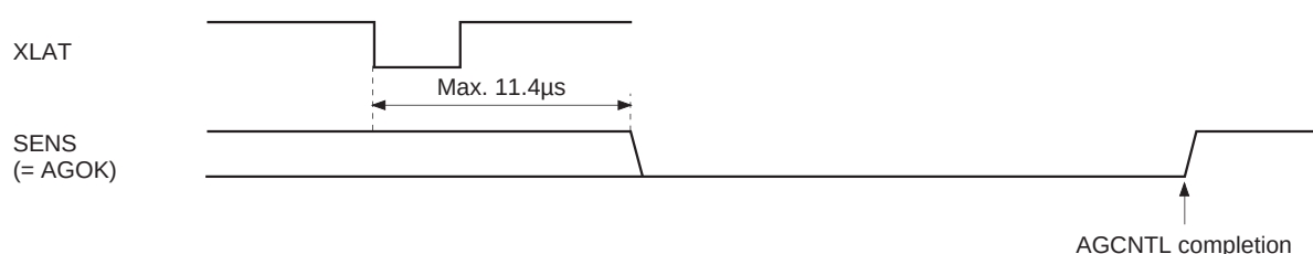
Timing Chart 4-4
