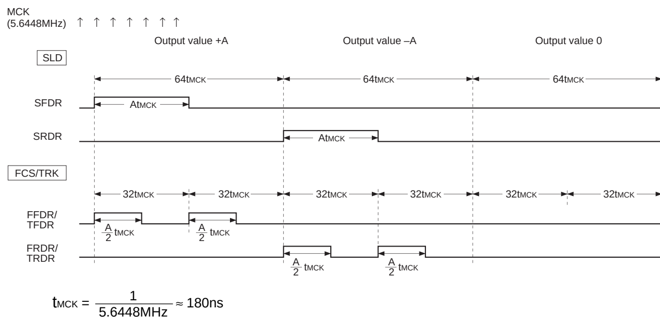
Timing Chart 4-20
