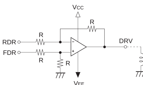
Fig. 4-21. Drive Circuit
