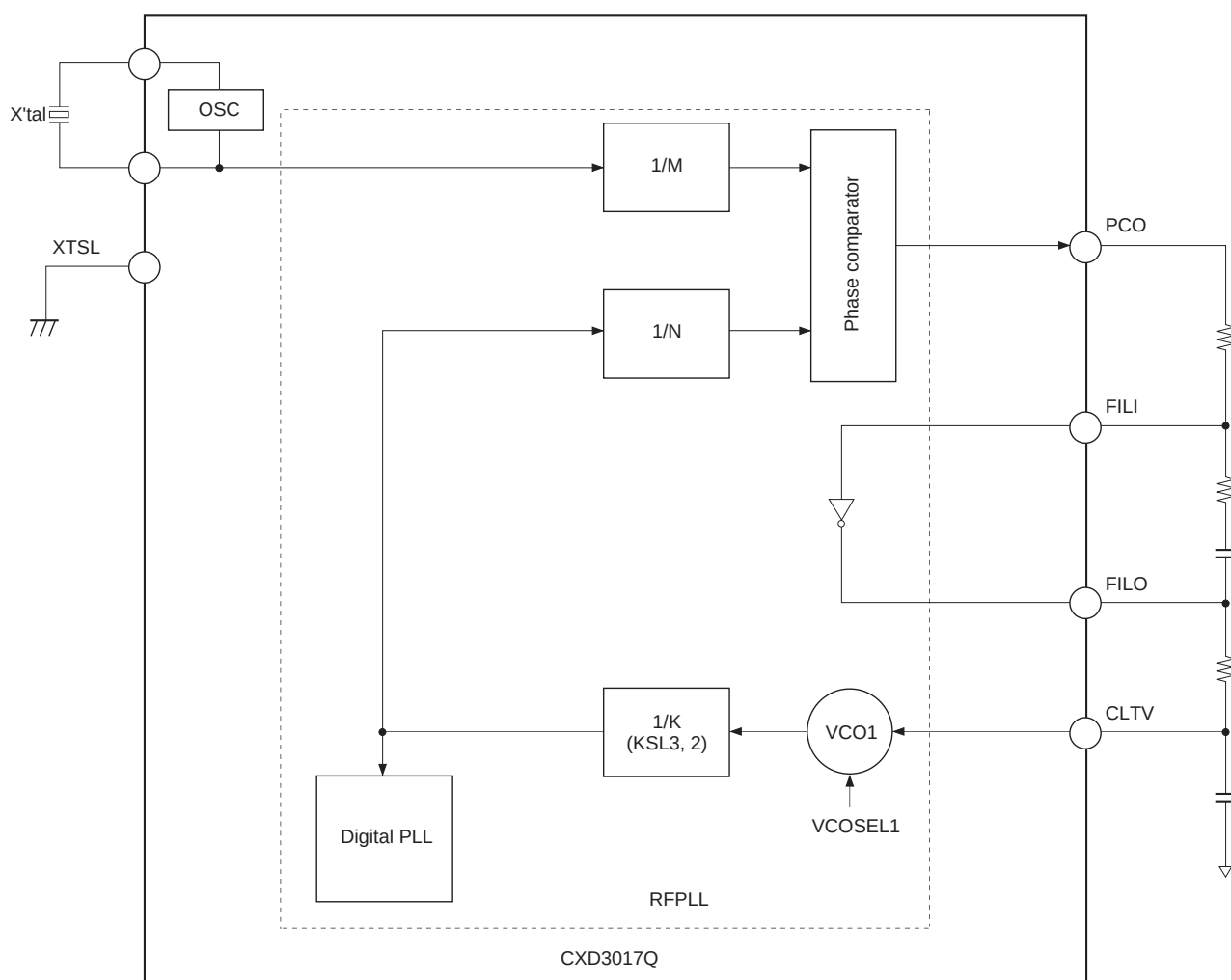
Block Diagram 3-1
