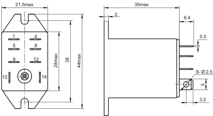
Outline Dimensions
