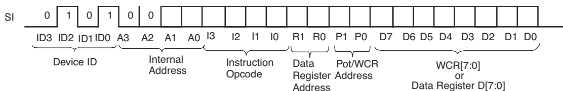
Figure 4. Three-Byte Instruction Sequence
