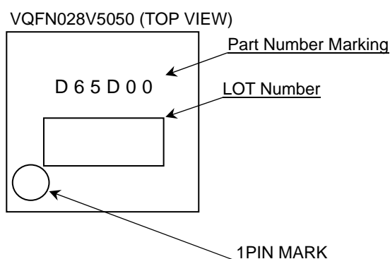
Figure 60. Marking Diagram
