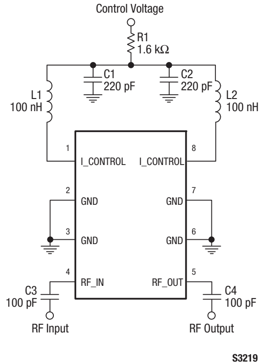
Figure 9. SKY12228-12LF Evaluation Board Schematic
