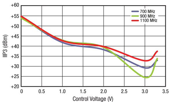
Figure 5. IIP3 vs Control Voltage vs Frequency (Spacing = 10 MHz)
