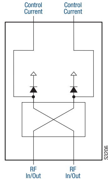
Figure 1. SKY12228-12LF Block Diagram
