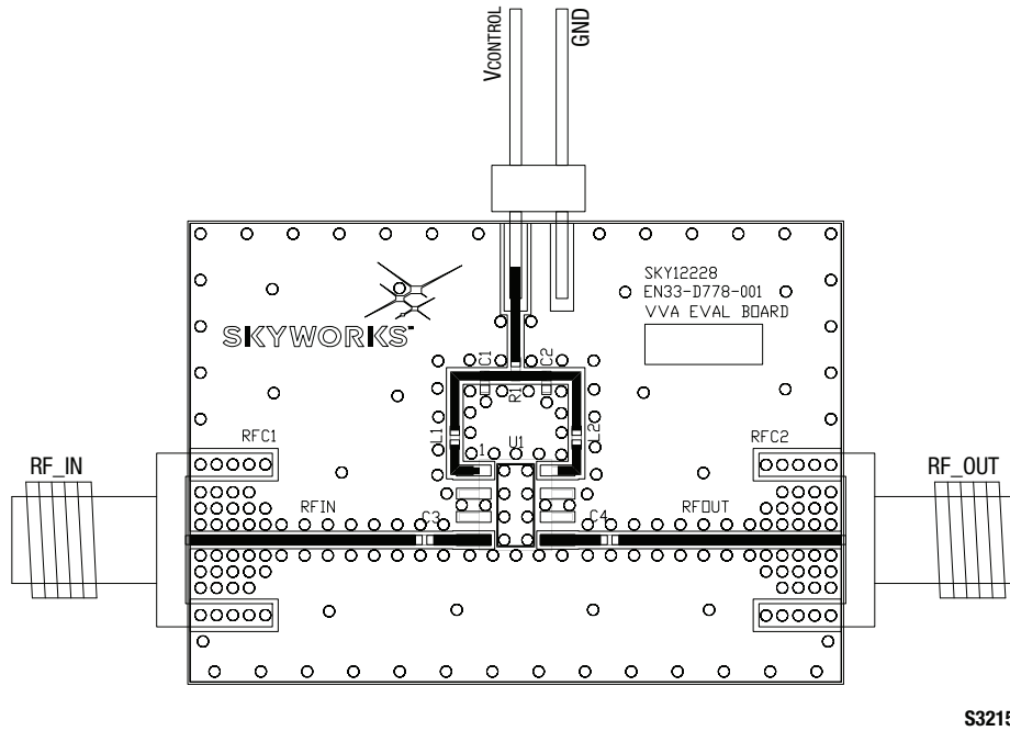
Figure 7. SKY12228-12LF Evaluation Board Assembly Diagram
