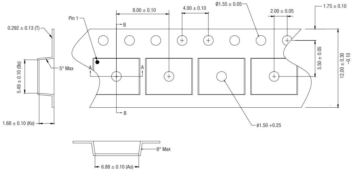
Figure 12. SKY12228-12LF 8-Pin SOIC Package Dimensions
