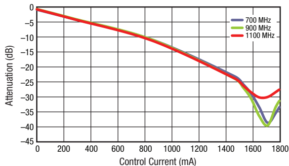
Figure 6. Attenuation vs Control Current vs Frequency
