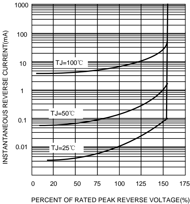
FIG.5-TYPICAL JUNCTION
