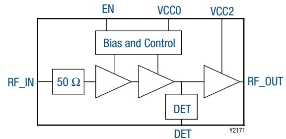
Figure 1. SE2623L-R Block Diagram
